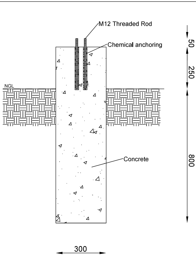
Section Detail
