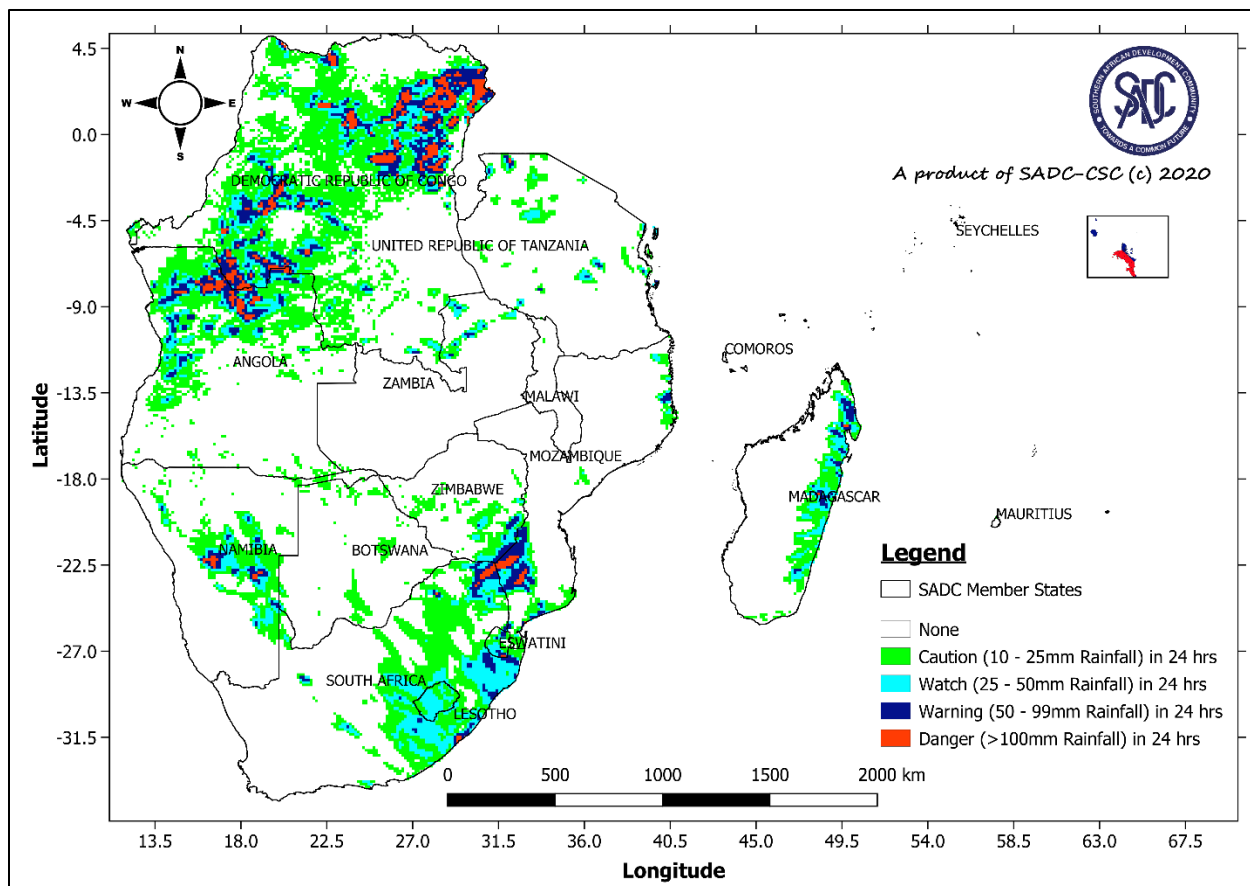
Figure 1: SADC Region's heavy rainfall advisory for the period 15 to 21 April 2020 (Source: SADC-CSC-WRF GFS Model)
