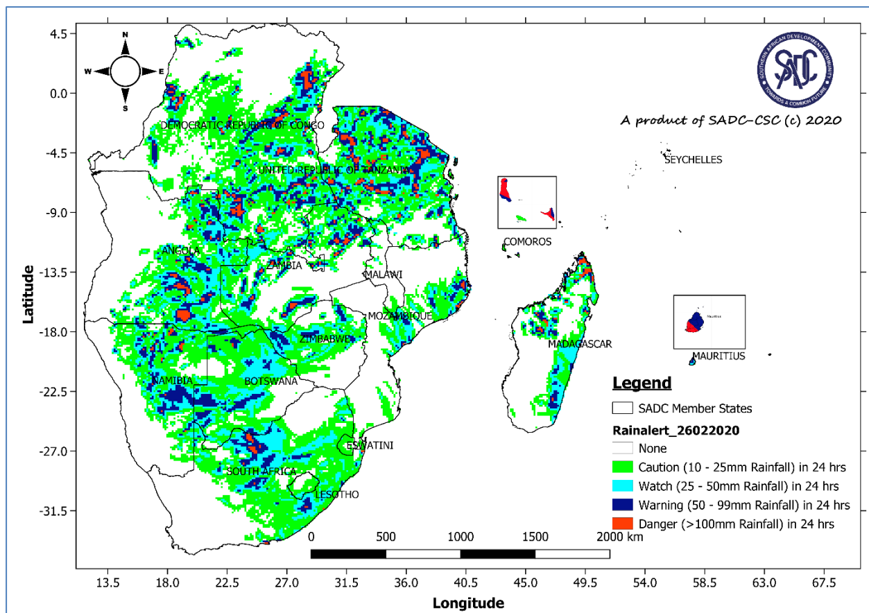
Figure 1: SADC Region's heavy rainfall advisory for the period 27 February to 04 March 2020 (Source: SADC-CSC-WRF GFS Model)
