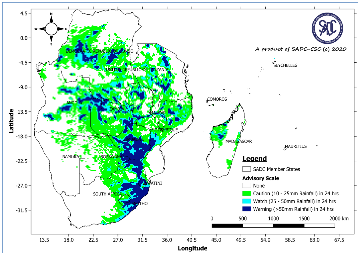
Figure 1: SADC Region's heavy rainfall advisory for the period 05 to 11 February 2020 (Source: SADC-CSC-WRF GFS Model)
